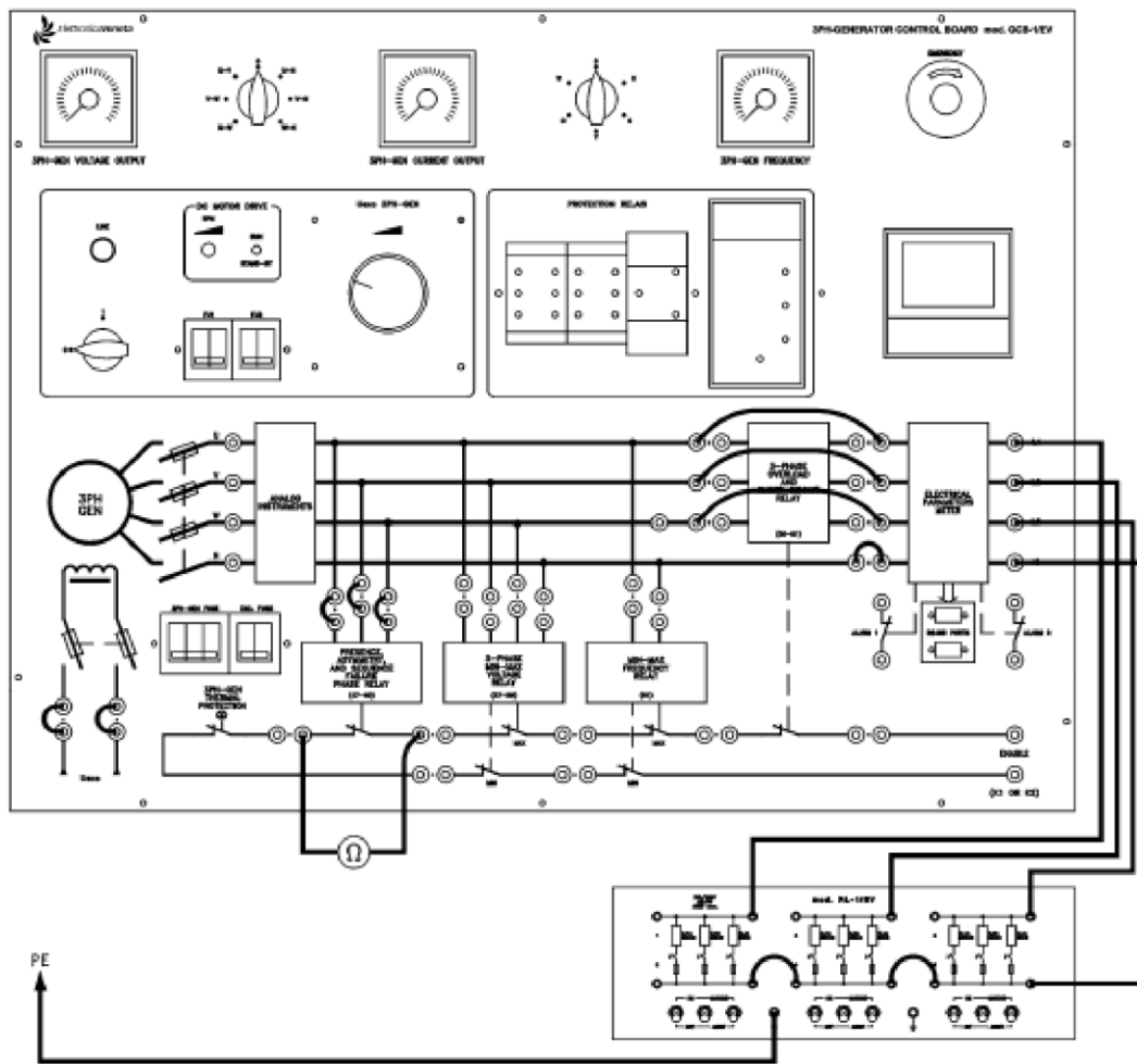
Connections on the board GCB-1/EV.
