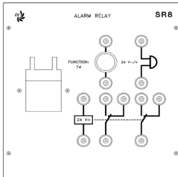
Figure 1: Alarm Relay
