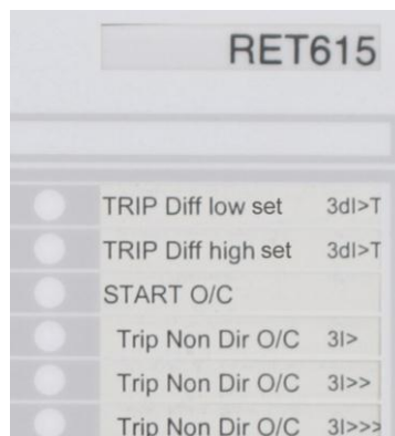
Fig. 12.8 Alarm indicator LEDs
