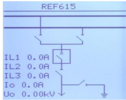
Fig. 10.2 Single Line Diagram (SLD) REF615
