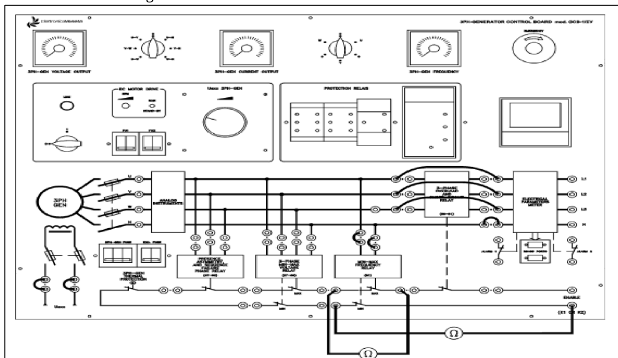
Connections on the board GCB-1/EV. Figure 2 Operation test of the max/min frequency relay.
