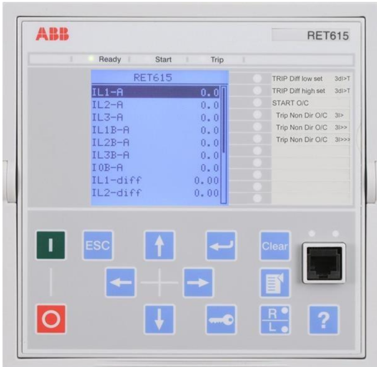
Fig. 12.4 Human Machine Interface RET615
