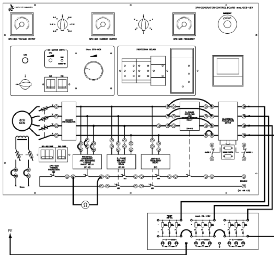
Figure 2 Operation test of the relay for phase sequence, phase lacking and voltage asymmetry
